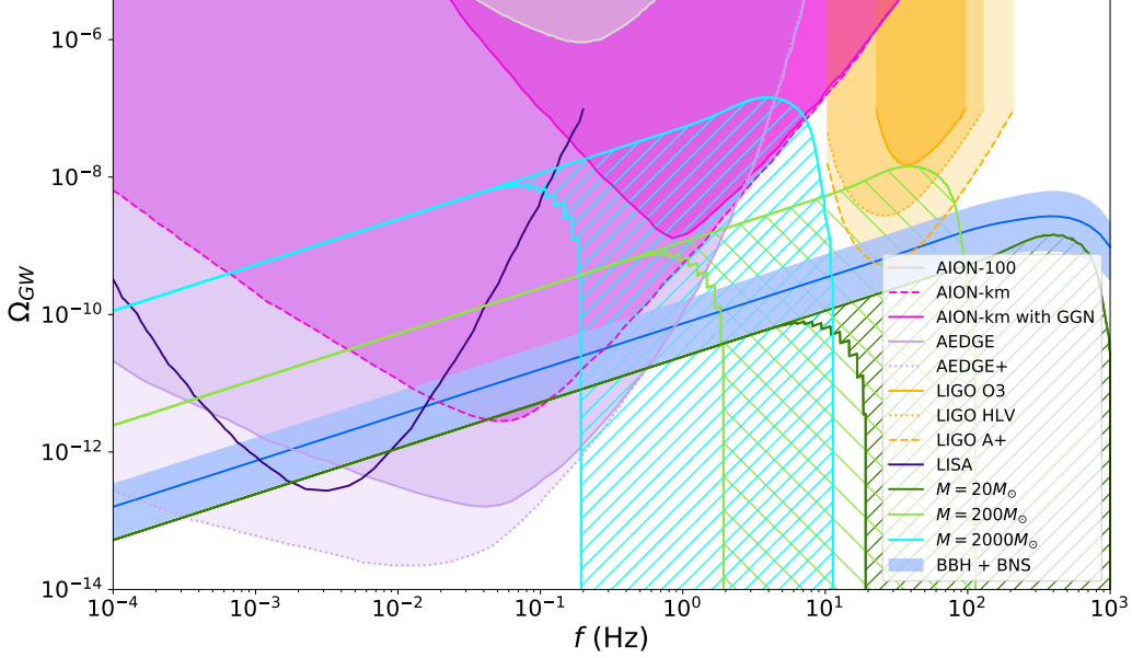
Figure 3. An estimation of the potential signal from mergers of populations of ECOs each of mass M/2 where M = 20, 200, 2000M_{\odot} is the total binary mass, assuming an identical redshift distribution to LIGO black holes and a present merger rate of 10 \text{ Gpc}^{-3} \text{ yr}^{-1} . The lower frequency cut-off of each band only includes only the inspiral phase, terminating at the ISCO frequency assuming a compactness scale of C = 0.1 . The higher frequency cut off additionally includes merger and ringdown phases, using the BH wavefunctions given in eq. 2.11. The cumulative GWB from BH and NS populations is shown as a solid blue line. The upper (lower) limits of the blue band are linear additions of the upper (lower) limits of each of these populations individually. The dashed red line is a conservative upper estimate of the total astrophysical signal, obtained by linearly adding the upper limits of each of the BH, NS and BHNS populations. Also shown are the power-integrated (PI) prospective sensitivities to stochastic (background) signals for the AION-100, AION-km, AEDGE and AEDGE+ experiments taken from Ref. [9]. We also display the predicted sensitivity for AION-km assuming that gravitational gradient noise (GGN) cannot be eliminated [9]. These estimates are based on Peterson’s new low noise model (NLNM) which bounds the expected seismically-induced GGN from below. The 2\sigma PI curves for the recent third LIGO observation run (O3), as well as projections for the HLV network and A+ detectors operating at design sensitivities are taken from [54], and the prospective sensitivity of LISA [73] to stochastic signals is taken from Ref. [42].
