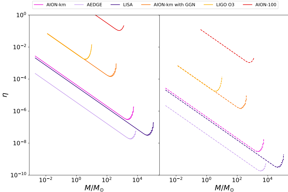
Figure 4. A plot of the minimum fraction \eta of dark matter required to be in populations of identical mass binary ECOs as a function of total binary mass M , in order for the GWB to intersect the sensitivity curve of various experiments as shown in Fig. 2. The left and right hand panels show the cases where the number of mergers occurring in one Hubble time correspond to 1%, and 100% of the total number of binary systems respectively i.e. \epsilon = 0.01 and \epsilon = 1 .
