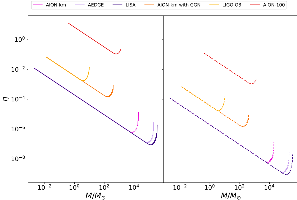
Figure 5. A plot of the minimum fraction \eta of dark matter required to be in populations of identical mass binary ECOs as a function of total binary mass M , in order for the GWB signal to both intersect the sensitivity curve of various experiments as shown in Fig. 2 and exceed the cumulative GWB from merging BH and NS (the solid blue line in Fig. 2). The left and right hand panels show the cases where the number of mergers occurring in one Hubble time correspond to 1%, and 100% of the total number of binary systems respectively i.e. \epsilon = 0.01 and \epsilon = 1 .
