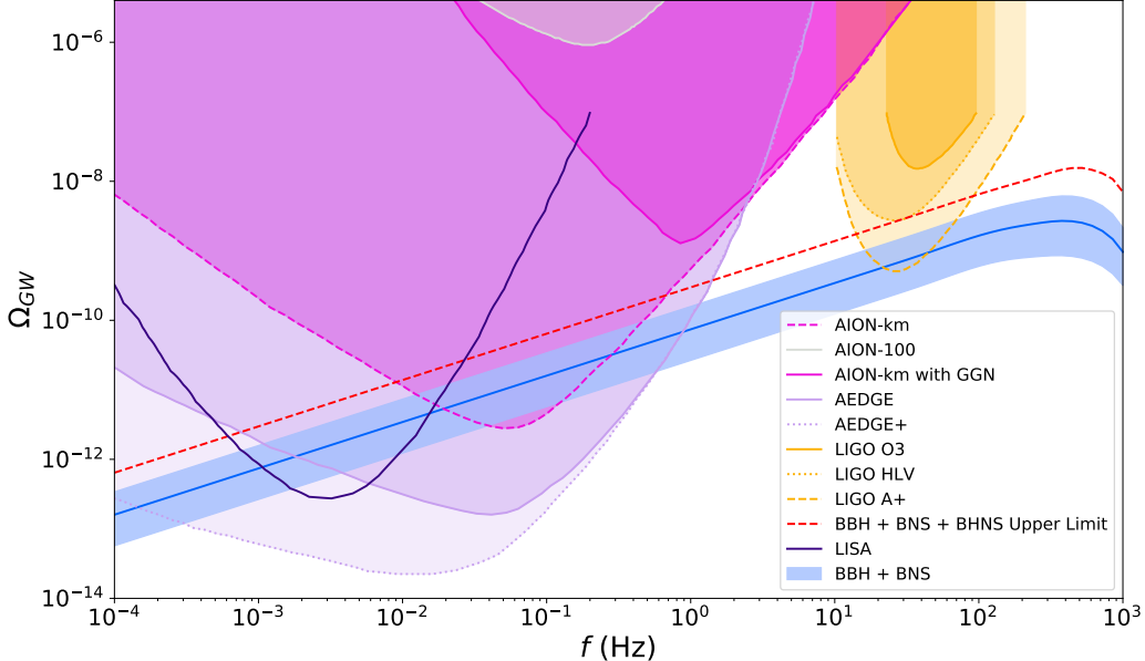
Figure 2. The total GWB from BH and NS populations is shown as a solid blue line. The upper (lower) limits of the blue band are linear additions of the upper (lower) limits of each of these populations individually. The dashed red line is a conservative upper estimate of the total astrophysical signal, obtained by linearly adding the upper limits of each of the BH, NS and BHNS populations. Also shown are the power-integrated (PI) prospective sensitivities to stochastic (used here to mean cumulative or background) signals for the AION-100, AION-km, AEDGE and AEDGE+ experiments taken from Ref. [9]. We also display the predicted sensitivity for AION-km assuming that gravitational gradient noise (GGN) cannot be eliminated [9]. These estimates are based on Peterson’s new low noise model (NLNM) which bounds the expected seismically-induced GGN from below. The 2\sigma PI curves for the recent third LIGO observation run (O3), as well as projections for the HLV network and A+ detectors operating at design sensitivities are taken from [54], and the prospective sensitivity of LISA [73] to stochastic signals is taken from Ref. [42].
