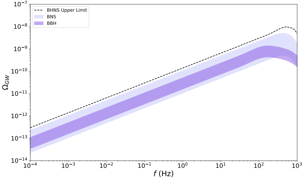
Figure 1. Estimates of the gravitational wave backgrounds from mergers of stellar-mass BH, NS and BHNS binaries. The signal from BH and NS binary populations are shown as bands whose upper (lower) values arise from adopting the 1\sigma upper (lower) limits of the present merger rate R_0 as extracted from LIGO-Virgo data in Ref. [58] and Ref. [12] respectively. The dashed line is a (conservative) upper estimate of the signal from BHNS mergers.
